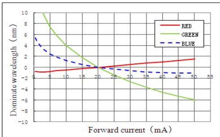
Dominate Wavelength VS Forward Current
